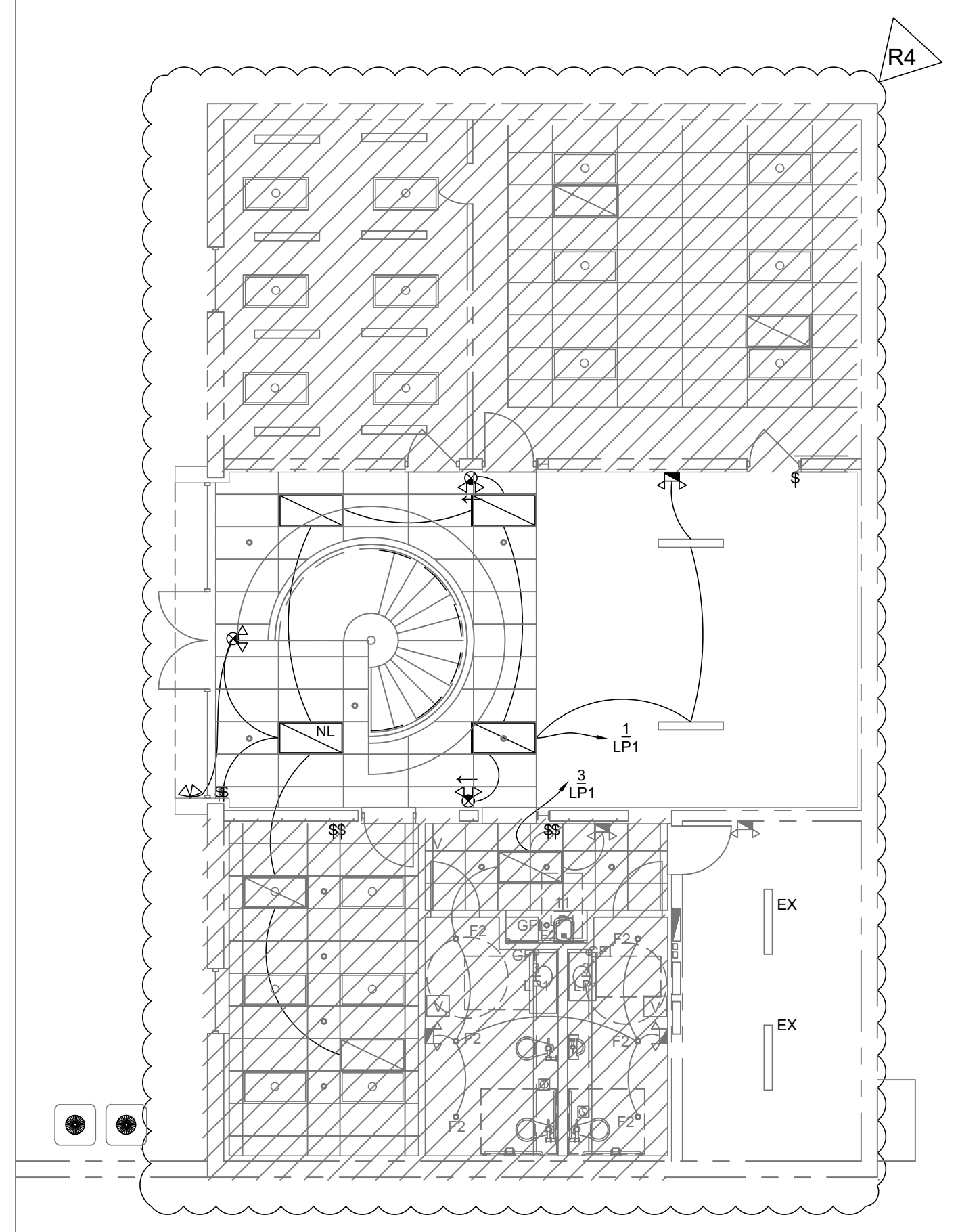
LOWER LEVEL LIGHTING LAYOUT SCALE: 1/8" = 1'-0"
