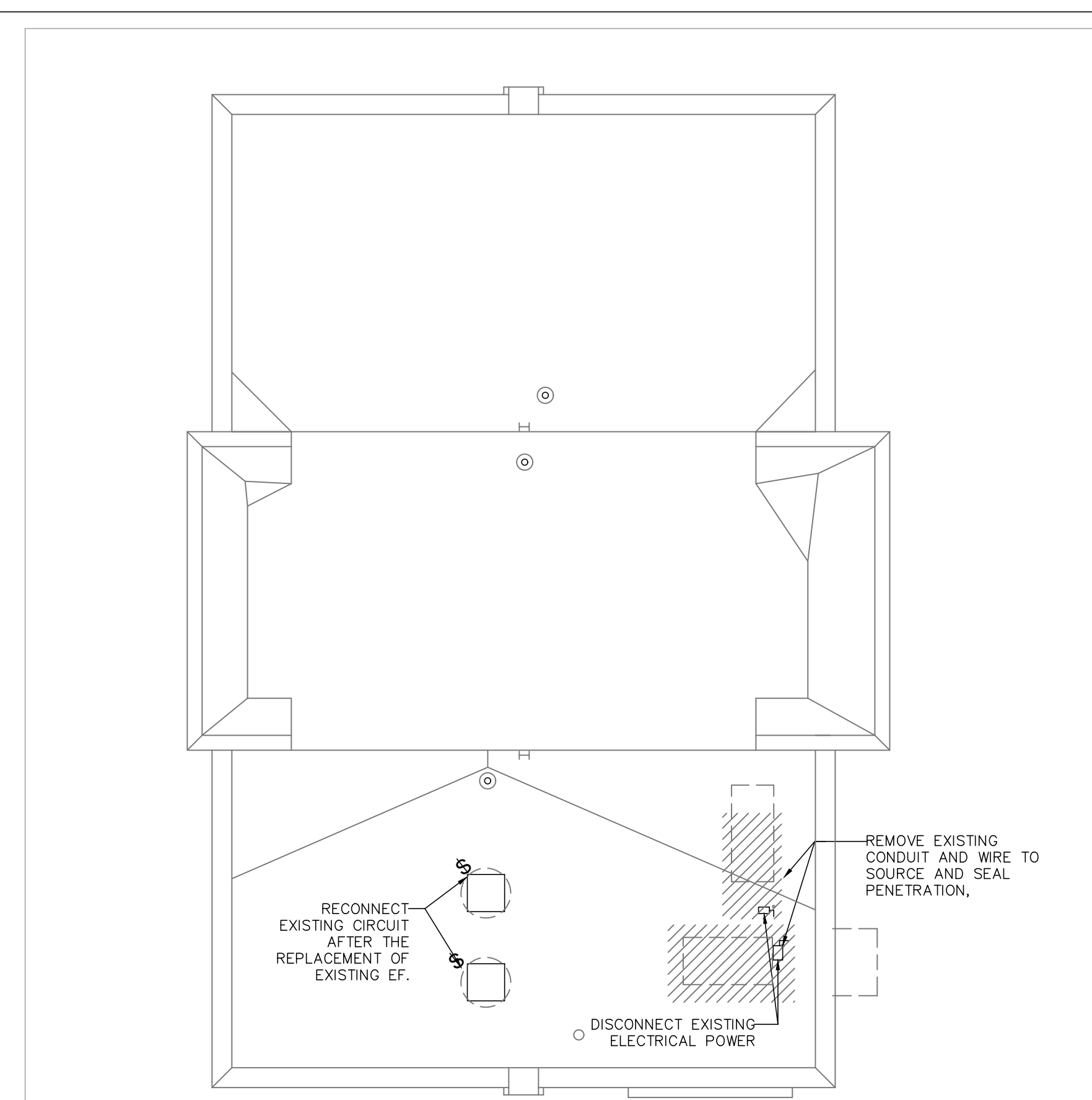
ROOF ELECTRICAL LAYOUT SCALE: 1/8" = 1'-0" MIRROR LINE
