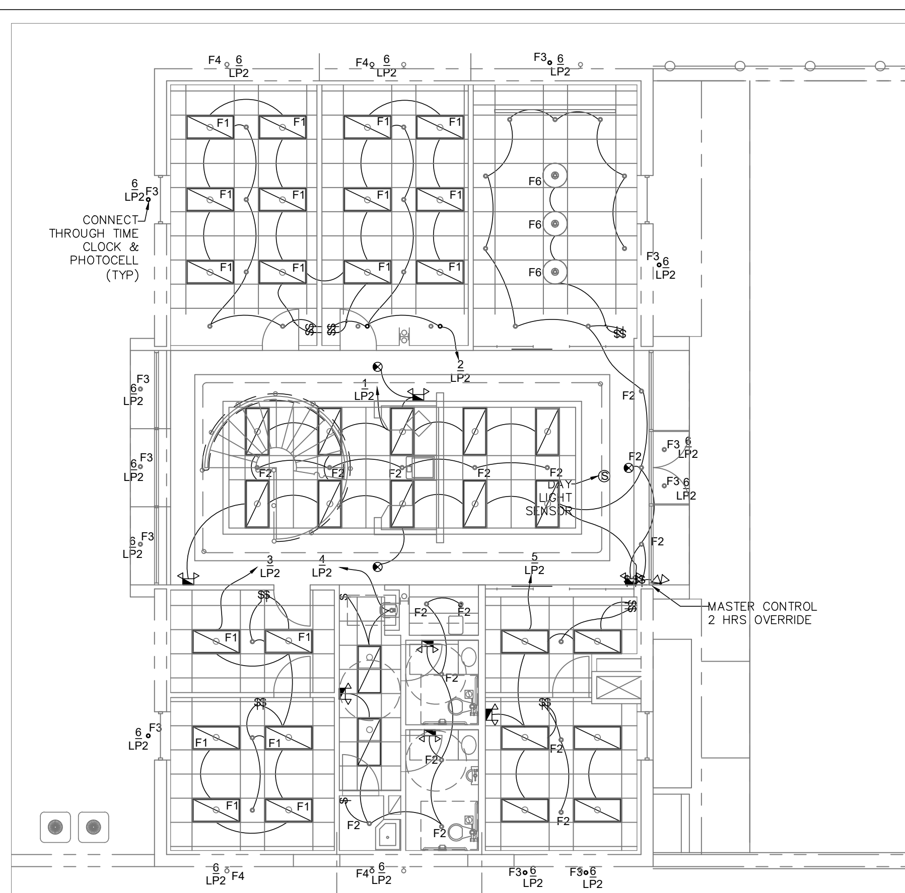
MAIN LEVEL LIGHTING LAYOUT SCALE: 1/8" = 1'-0"
