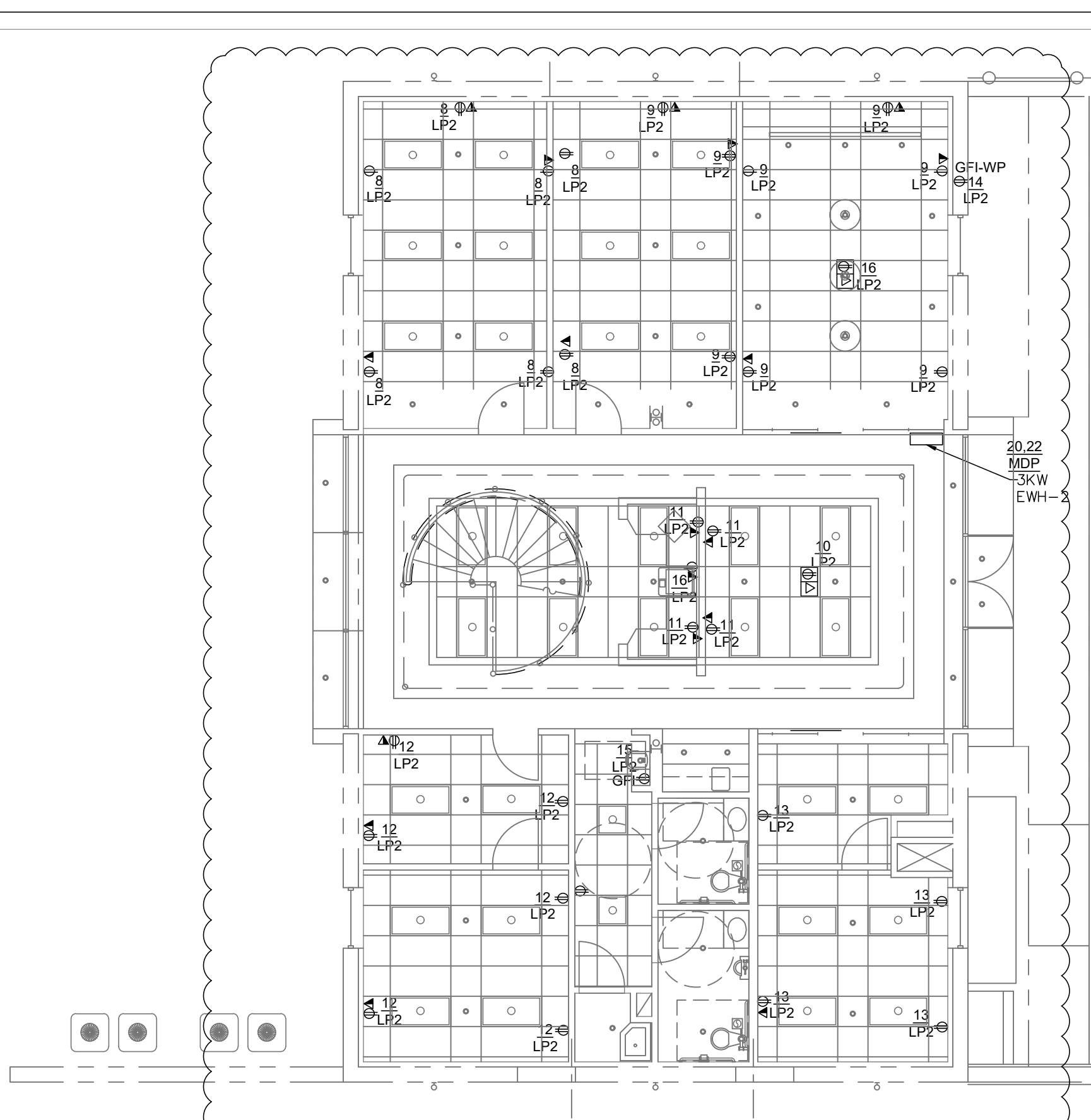
MAIN LEVEL POWER LAYOUT SCALE: 1/8" = 1'-0"
