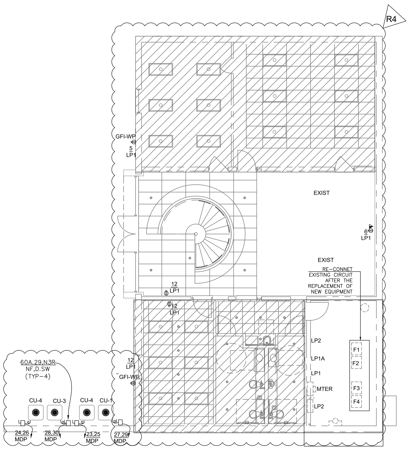
MAIN LEVEL POWER LAYOUT SCALE: 1/8" = 1'-0"
